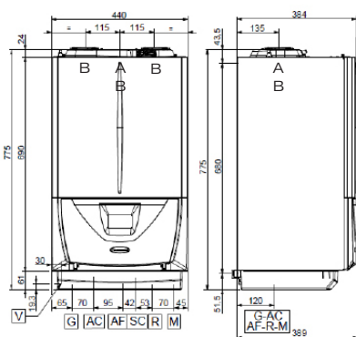
VICTRIX SUPERIOR 26
